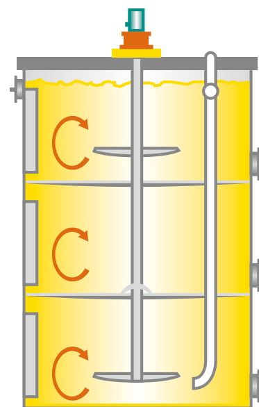
Recausticizing tank
