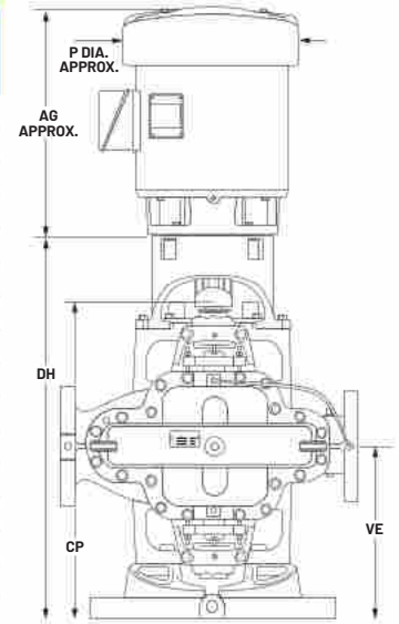
MODELS 1810 AND 1840
