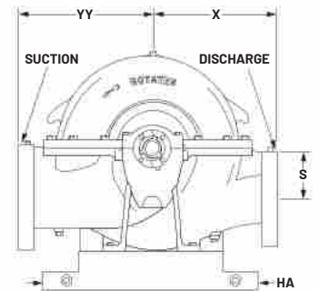
MODELS 1810 AND 1840
